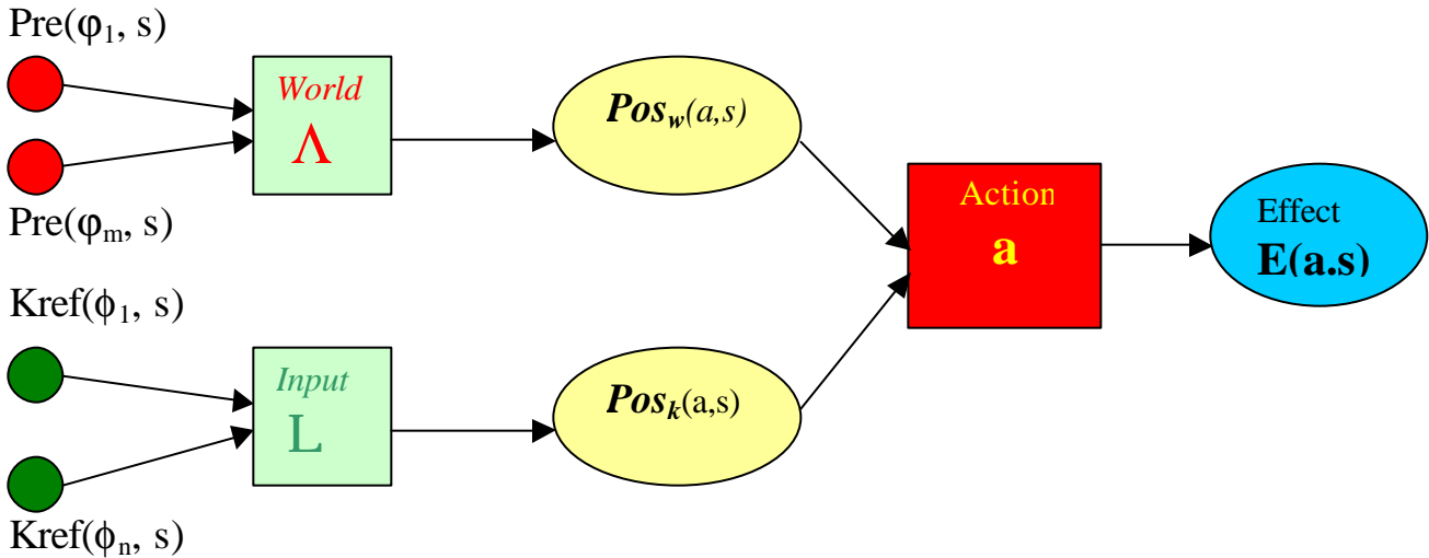
Figure 1. Atomic DAML-S process
