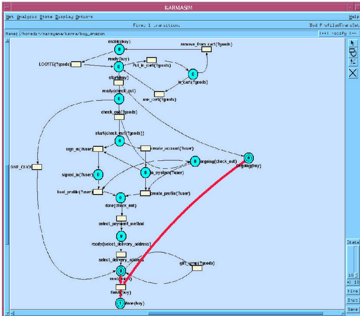
Figure 4. KarmaSIM simulation the DAML-S congo example
