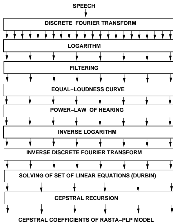
Figure 1: RASTA-PLP Method
