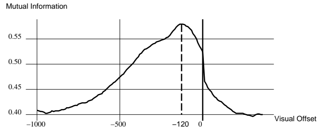
Figure 4: Cross-modal mutual information measurements. The X-axis shows the the visual to acoustic offset and the Y-axis shows the cross-modal mutual information
