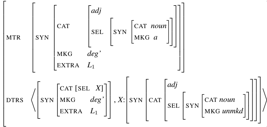
Figure 4: Complex Pre-Determiner Construction
