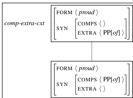
Figure 6: A Complement Extrapolation Construct
