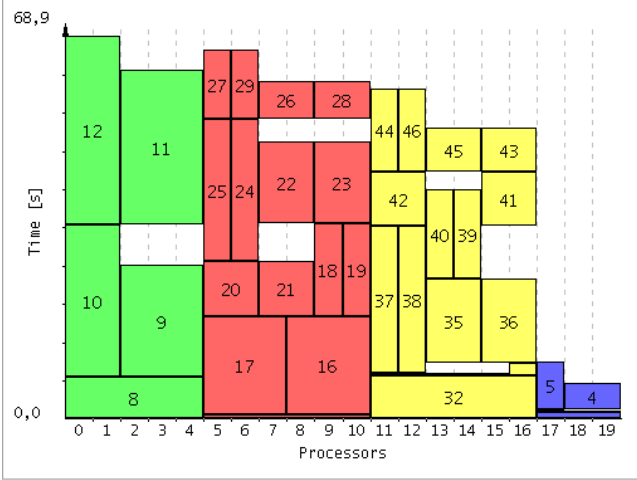
Figure 5. Jedule output for the schedule produced by the CRA_WIDTH algorithm. Four mixed-parallel applications, each having its own color, are scheduled on a cluster of 20 processors. The resource constraints imposed by the algorithm are respected.
