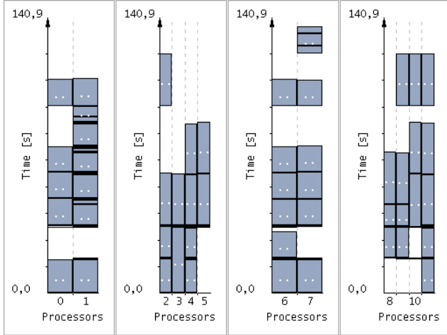
Figure 8. Jedule output of the schedule of a Montage instance on the heterogeneous platform described by Figure 7.
