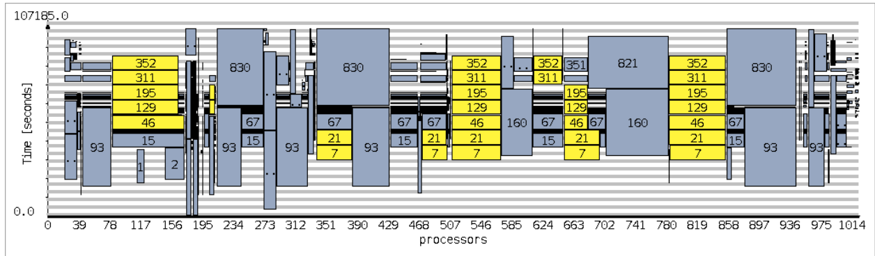
Figure 13. Visualization of the parallel workload of the LLNL Thunder Cluster on one day in 2007. Yellow rectangles denote jobs of a selected user.
