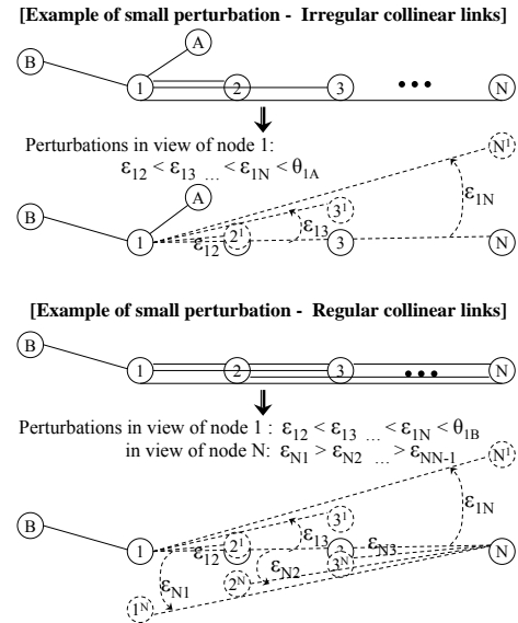
Figure 19: Examples of small perturbation.
