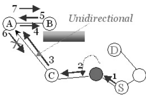
Figure 7: Routing failure caused by unidirectional links.
