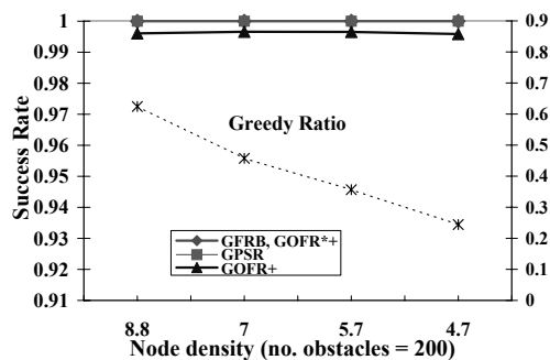
Figure 22: Success rate of four kinds of face routing combined with greedy routing.
