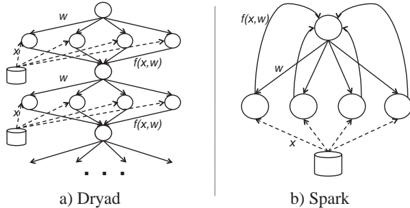
Figure 4: Data flow of a logistic regression job in Dryad vs. Spark. Solid lines show data flow within the framework. Dashed lines show reads from a distributed file system. Spark reuses processes across iterations, only loading data once.
