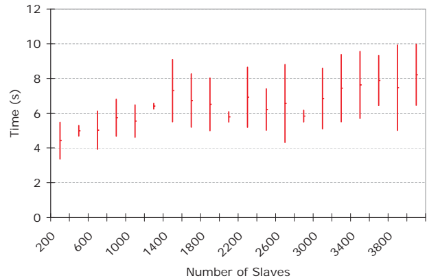
Figure 10: Mean time for the slaves and applications to reconnect to a secondary Mesos master upon master failure. The plot shows 95% confidence intervals.
