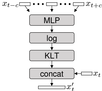
Figure 1: Tandem feature extraction: a multi-layer perceptron estimates phone posterior probabilities, which are transformed for better Gaussian modeling, then concatenated with a standard ASR feature vector to serve as an HMM’s acoustic observations.
