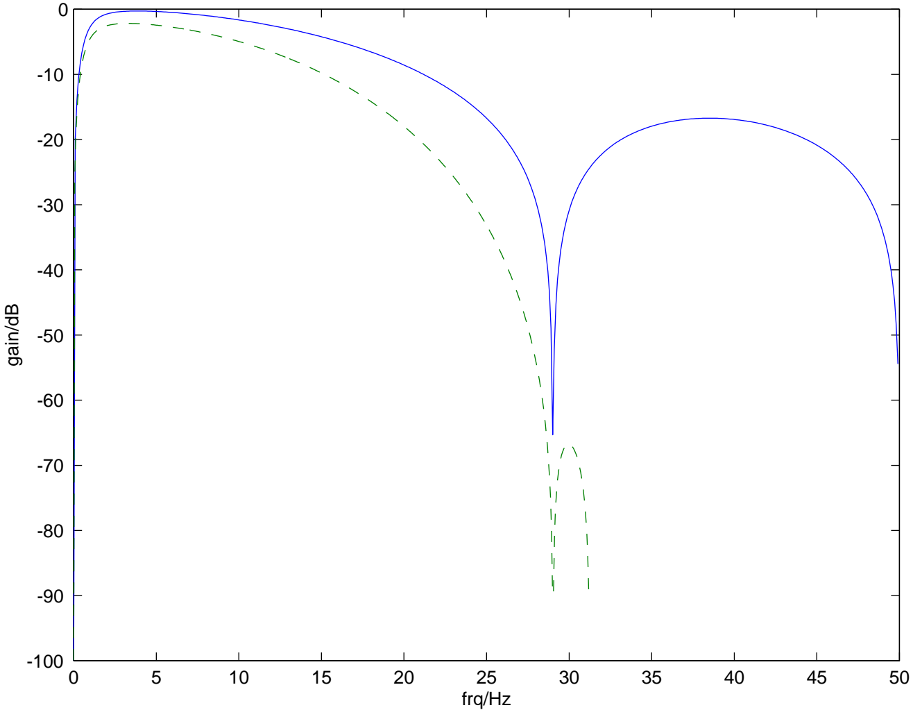
RASTA filter frequency response for 10 (-) and 16 (- -) ms frame steps
