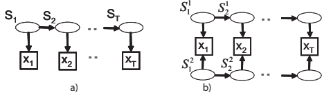
Fig. 2. a) Standard HMM and b) Factorial HMM.
